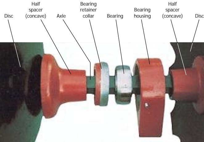
Exploded view of disc cultivator bearings
