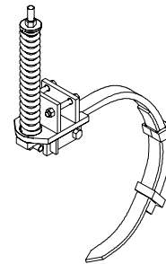
CP chisel tyne with feed down point
